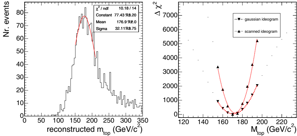
Figure 8.7. Distribution of the mass of the hadronic decaying top quark before the kinematic fit used for the \hat{M}_t^{fit} estimator (left) and the combined \Delta\chi^2(M_t) function over all events for both ideogram based estimators \hat{M}_t^{ParIdeo} and \hat{M}_t^{FullIdeo} (right).
